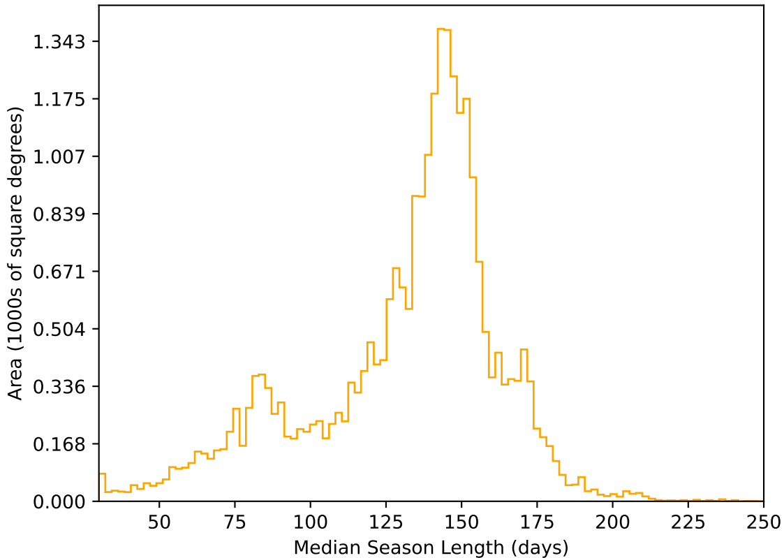
too_elab_r16_d3_giz_v3.4_10yrs All sky r band: Median Season Length
