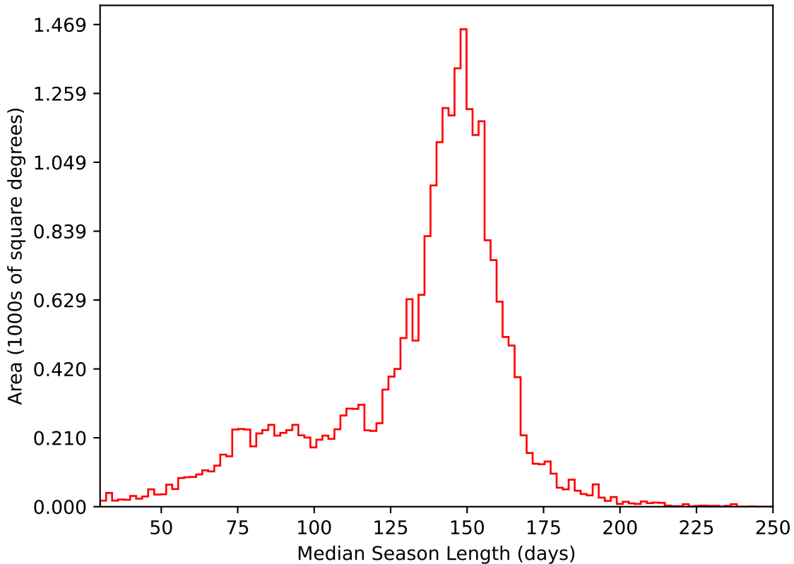
too_elab_r16_d3_giz_v3.4_10yrs All sky i band: Median Season Length
