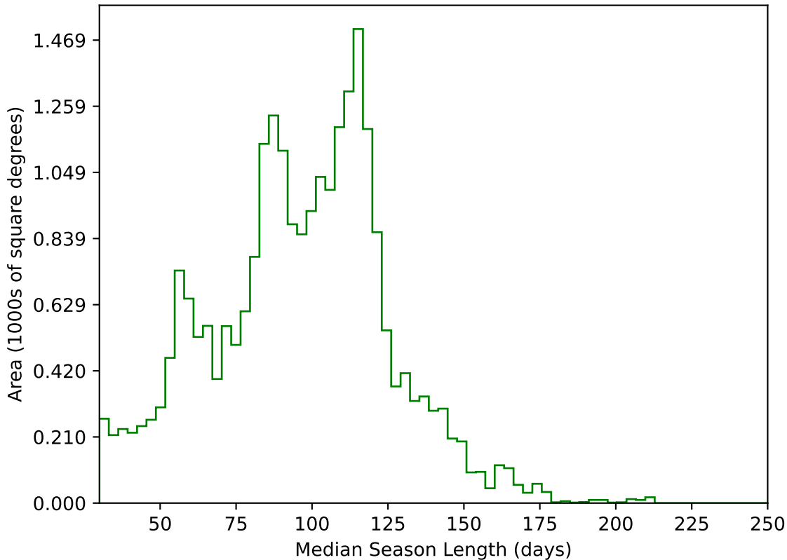
too_elab_r16_d3_giz_v3.4_10yrs All sky g band: Median Season Length
