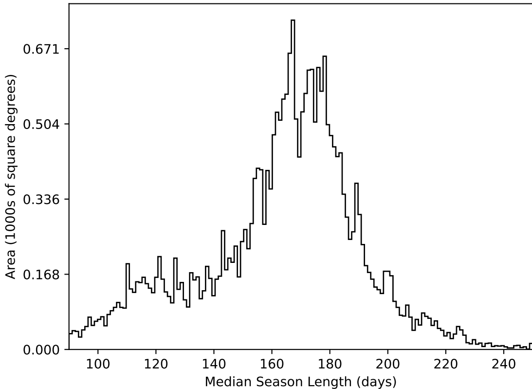
too_elab_r16_d3_giz_v3.4_10yrs All sky all bands: Median Season Length
