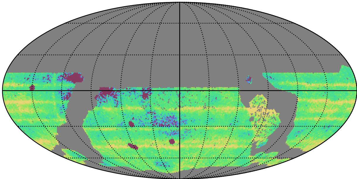
too_elab_r16_d3_giz_v3.4_10yrs WFD: Median Intra-Night Gap
