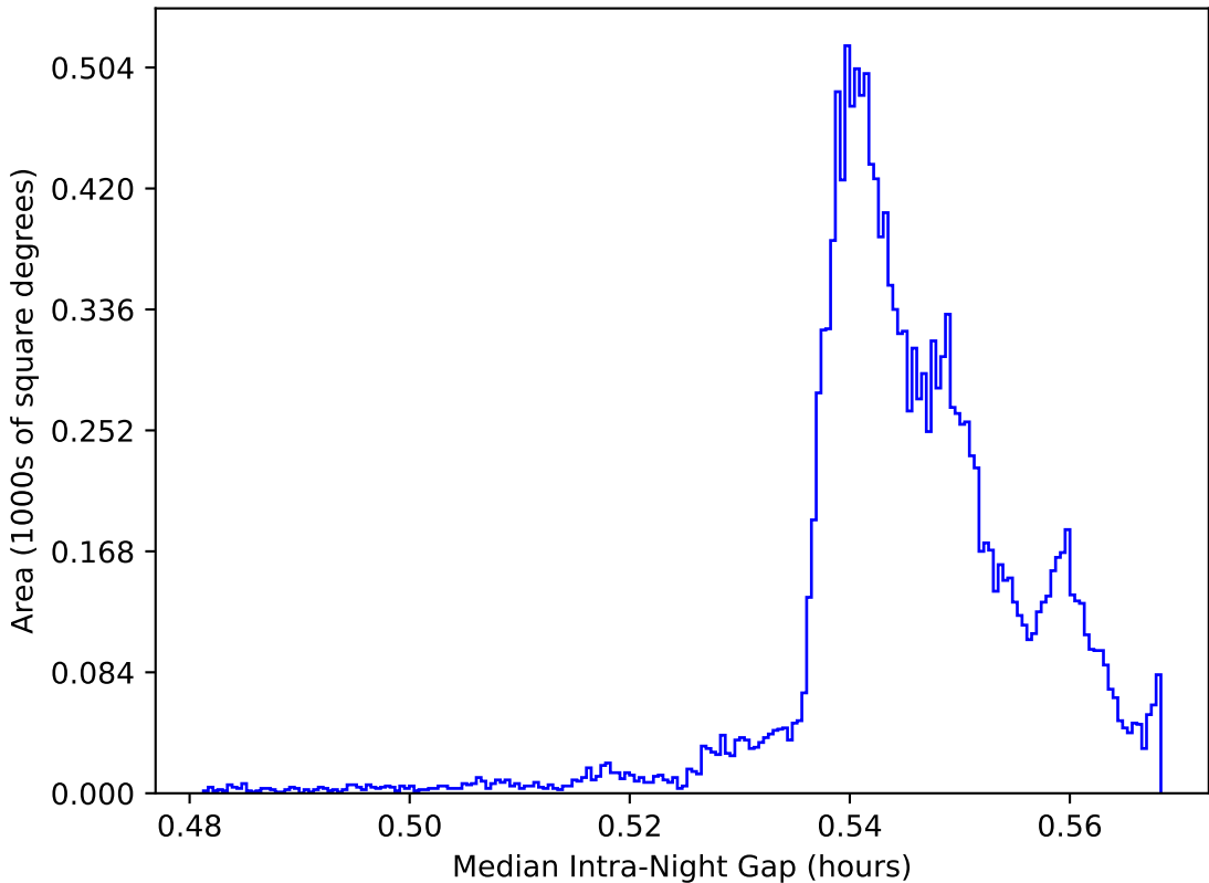
too_elab_r16_d3_giz_v3.4_10yrs WFD: Median Intra-Night Gap
