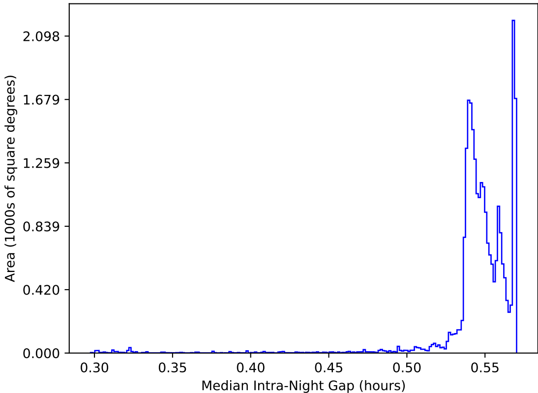
too_elab_r16_d3_giz_v3.4_10yrs All sky: Median Intra-Night Gap
