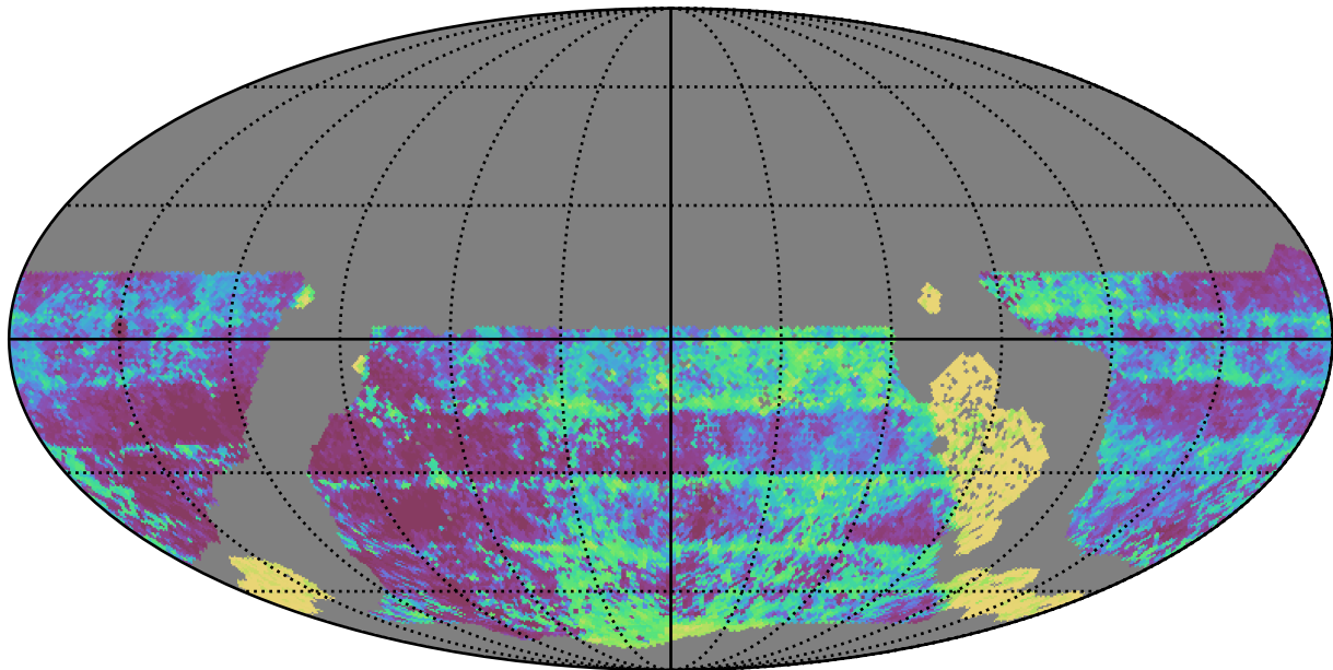
too_elab_r16_d3_giz_v3.4_10yrs WFD y band: Median Inter-Night Gap
