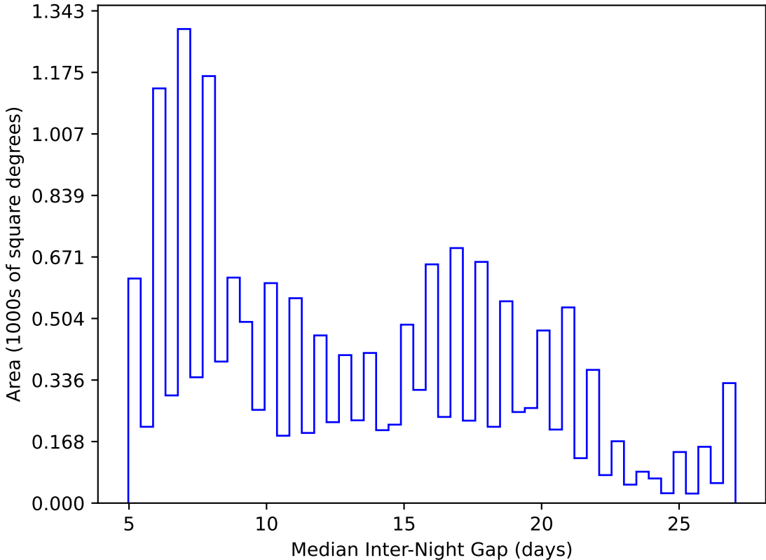
too_elab_r16_d3_giz_v3.4_10yrs WFD y band: Median Inter-Night Gap
