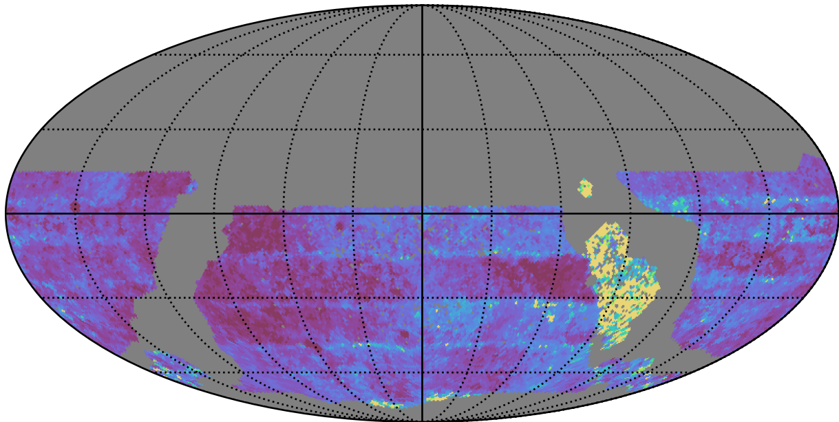
too_elab_r16_d3_giz_v3.4_10yrs WFD u band: Median Inter-Night Gap
