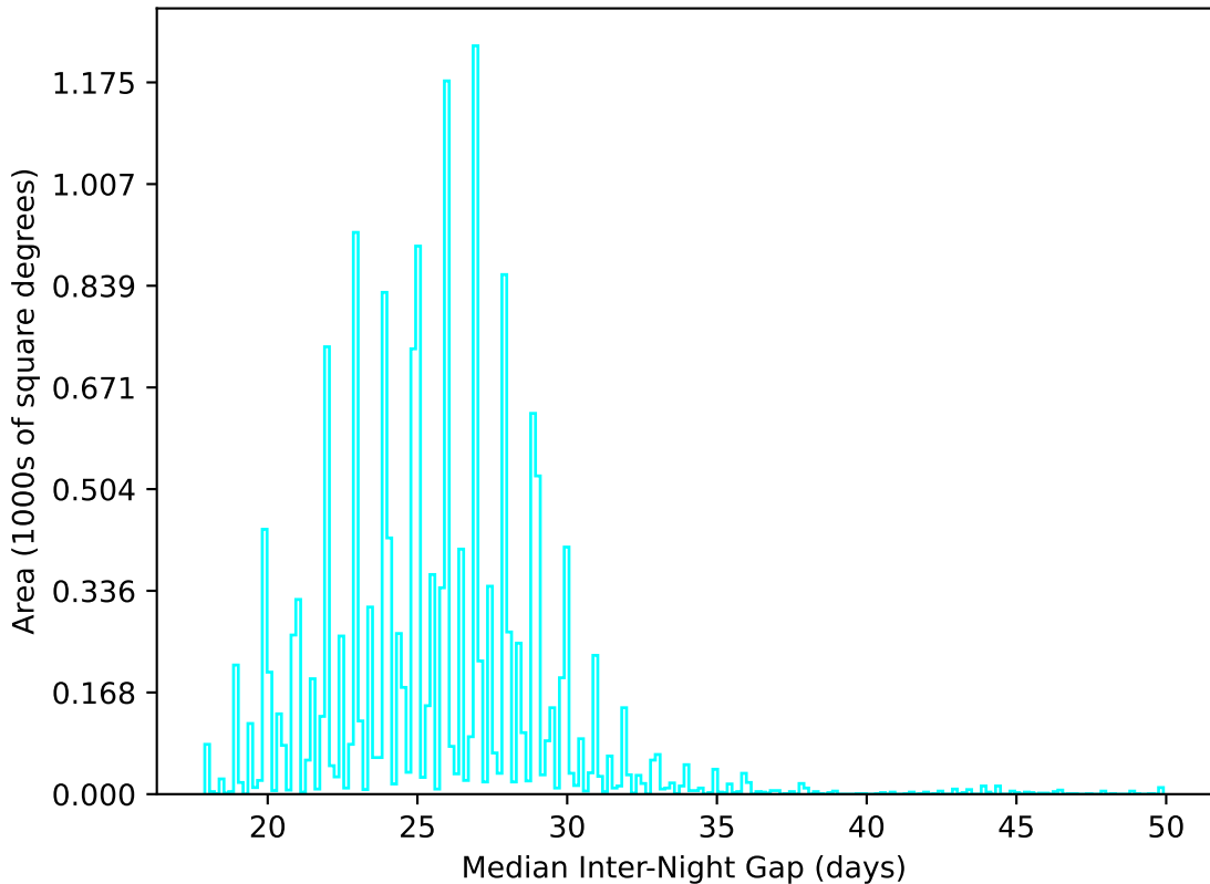
too_elab_r16_d3_giz_v3.4_10yrs WFD u band: Median Inter-Night Gap
