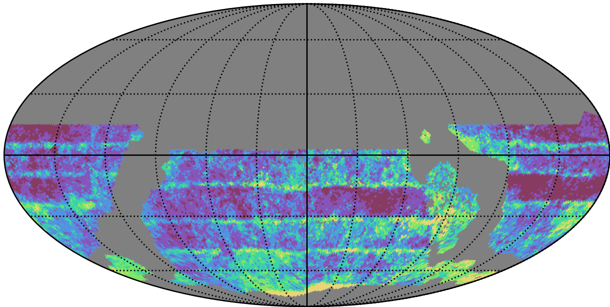
too_elab_r16_d3_giz_v3.4_10yrs WFD r band: Median Inter-Night Gap
