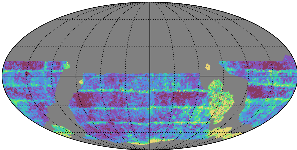
too_elab_r16_d3_giz_v3.4_10yrs WFD i band: Median Inter-Night Gap
