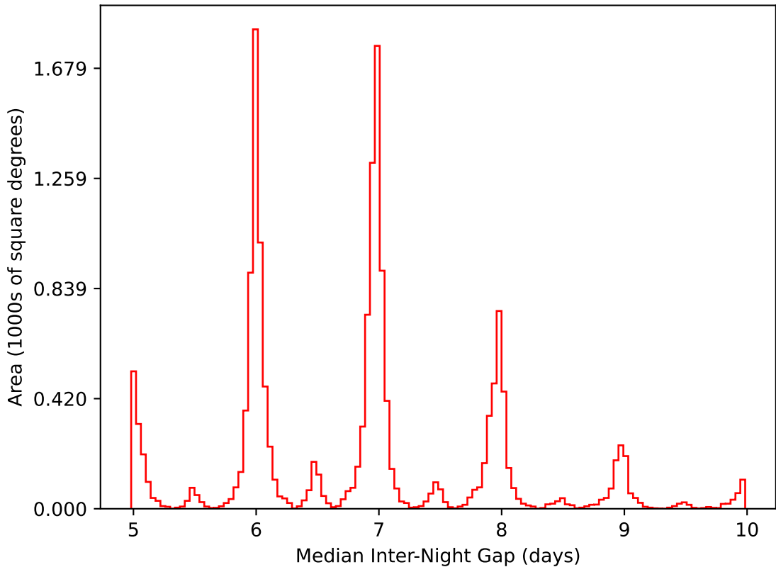
too_elab_r16_d3_giz_v3.4_10yrs WFD i band: Median Inter-Night Gap
