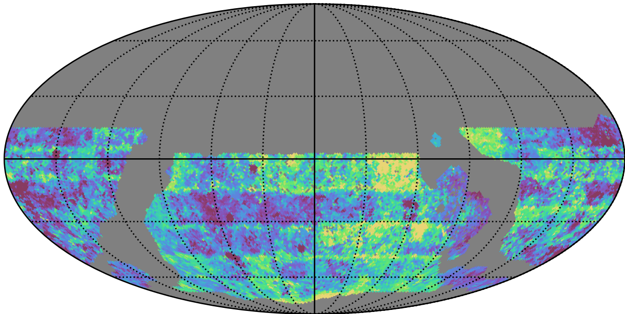
too_elab_r16_d3_giz_v3.4_10yrs WFD g band: Median Inter-Night Gap
