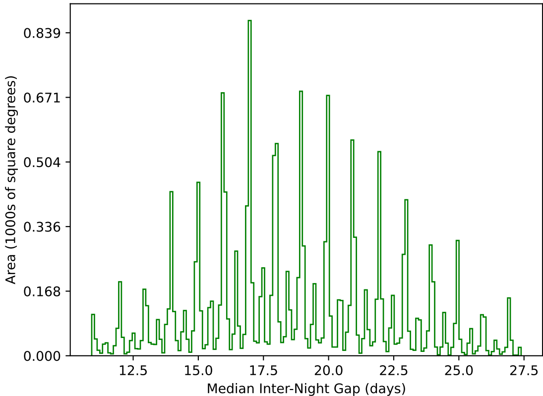
too_elab_r16_d3_giz_v3.4_10yrs WFD g band: Median Inter-Night Gap
