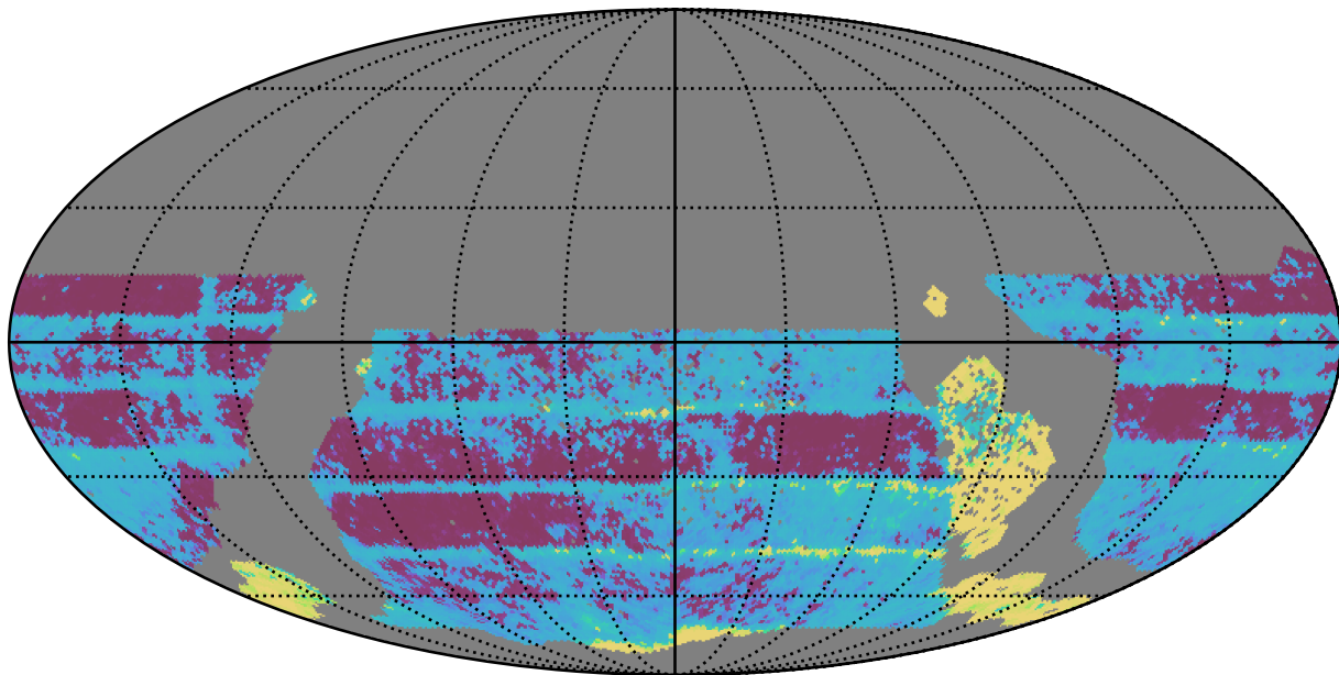
too_elab_r16_d3_giz_v3.4_10yrs WFD all bands: Median Inter-Night Gap
