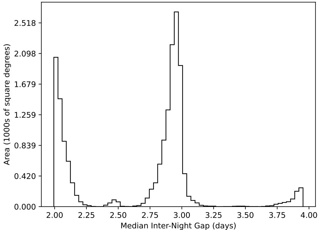
too_elab_r16_d3_giz_v3.4_10yrs WFD all bands: Median Inter-Night Gap
