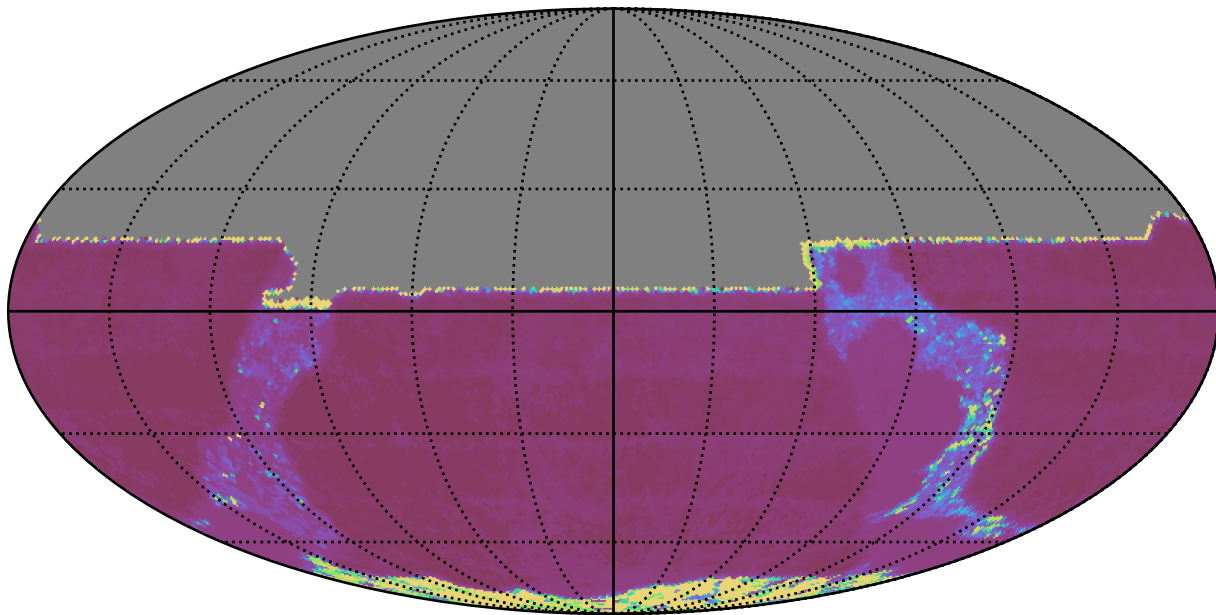
too_elab_r16_d3_giz_v3.4_10yrs All sky y band: Median Inter-Night Gap
