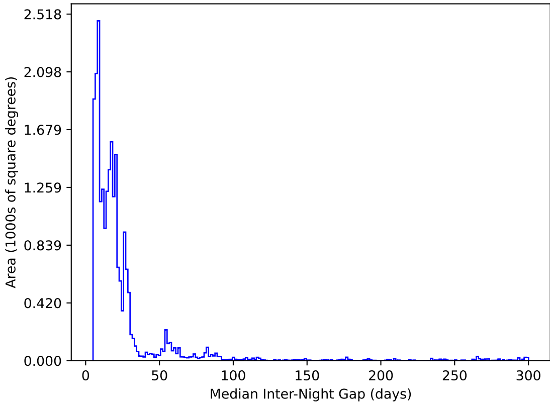
too_elab_r16_d3_giz_v3.4_10yrs All sky y band: Median Inter-Night Gap
