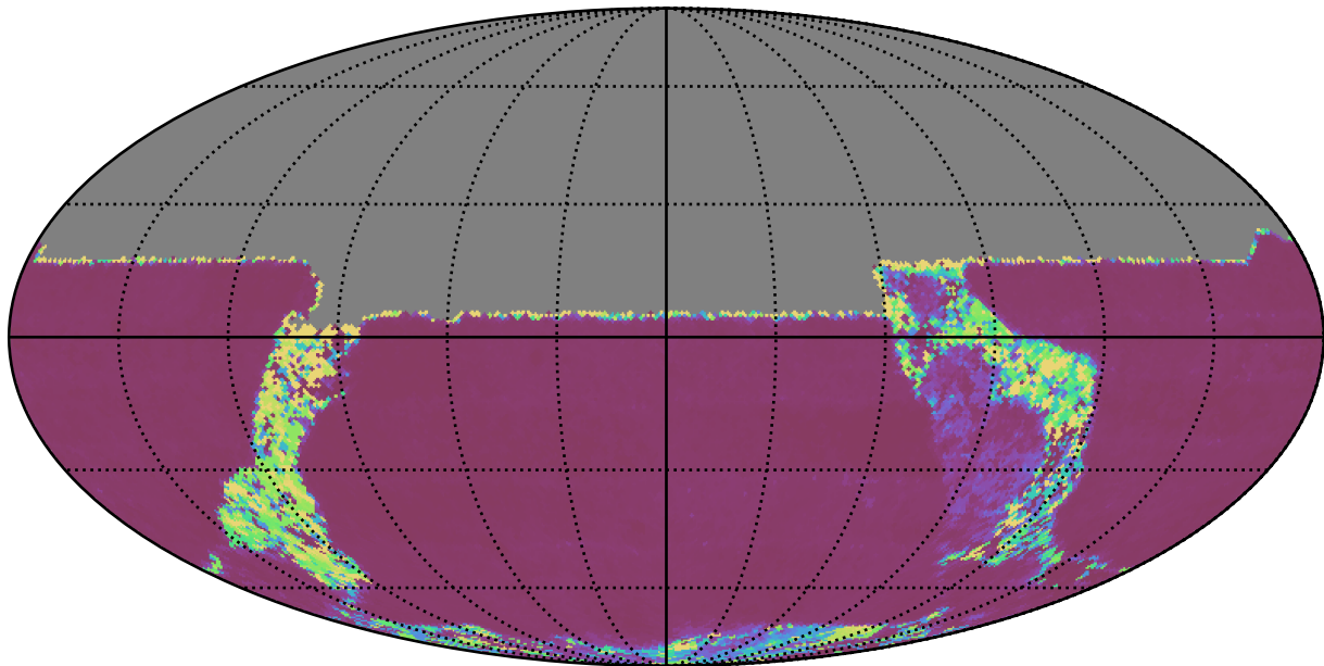
too_elab_r16_d3_giz_v3.4_10yrs All sky u band: Median Inter-Night Gap
