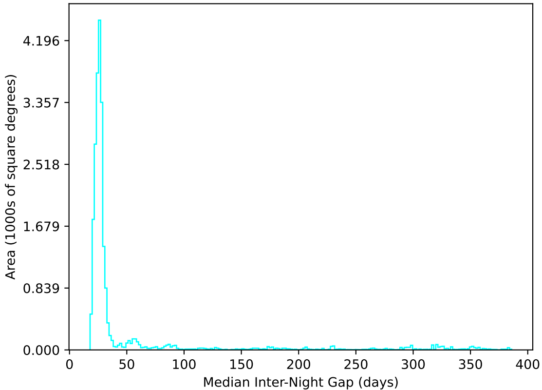
too_elab_r16_d3_giz_v3.4_10yrs All sky u band: Median Inter-Night Gap
