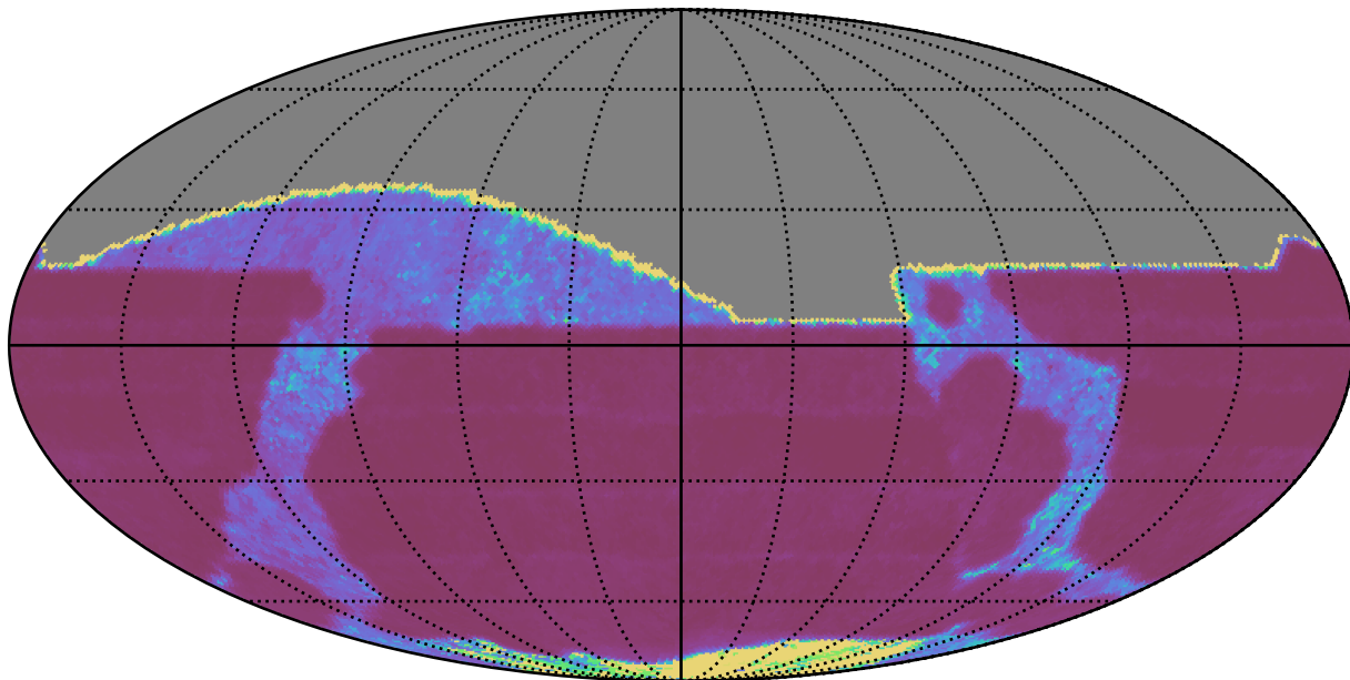
too_elab_r16_d3_giz_v3.4_10yrs All sky r band: Median Inter-Night Gap
