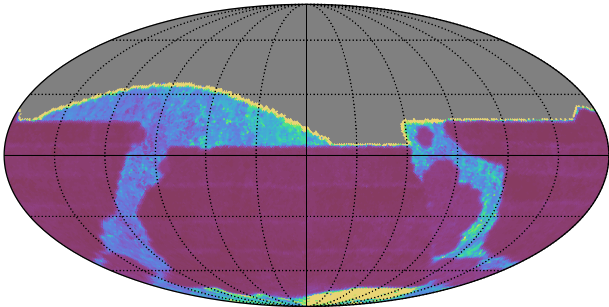
too_elab_r16_d3_giz_v3.4_10yrs All sky i band: Median Inter-Night Gap
