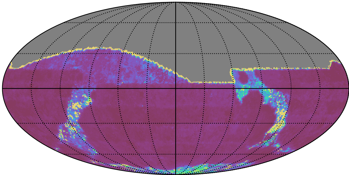
too_elab_r16_d3_giz_v3.4_10yrs All sky g band: Median Inter-Night Gap
