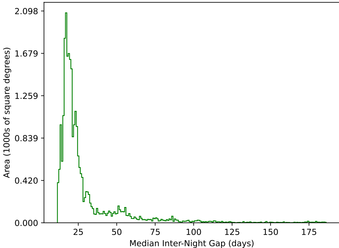
too_elab_r16_d3_giz_v3.4_10yrs All sky g band: Median Inter-Night Gap
