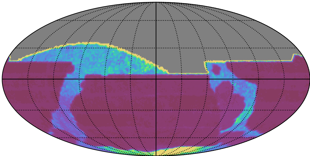
too_elab_r16_d3_giz_v3.4_10yrs All sky all bands: Median Inter-Night Gap
