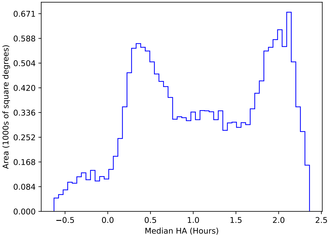
too_elab_r16_d3_giz_v3.4_10yrs WFD z band: Median HA
