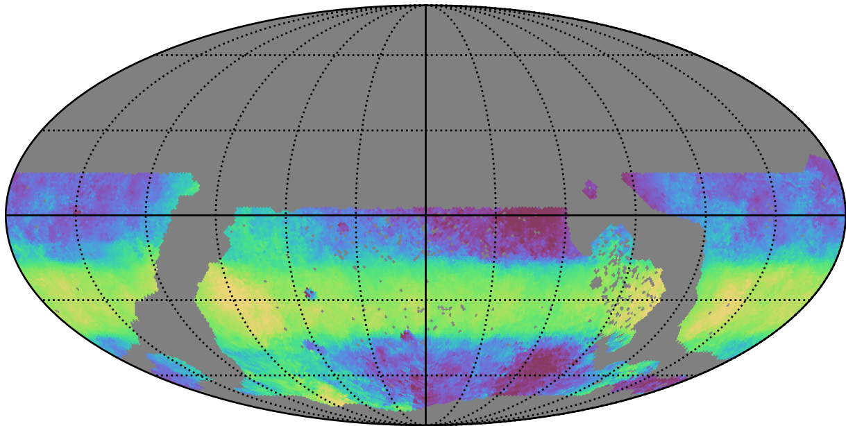
too_elab_r16_d3_giz_v3.4_10yrs WFD y band: Median HA
