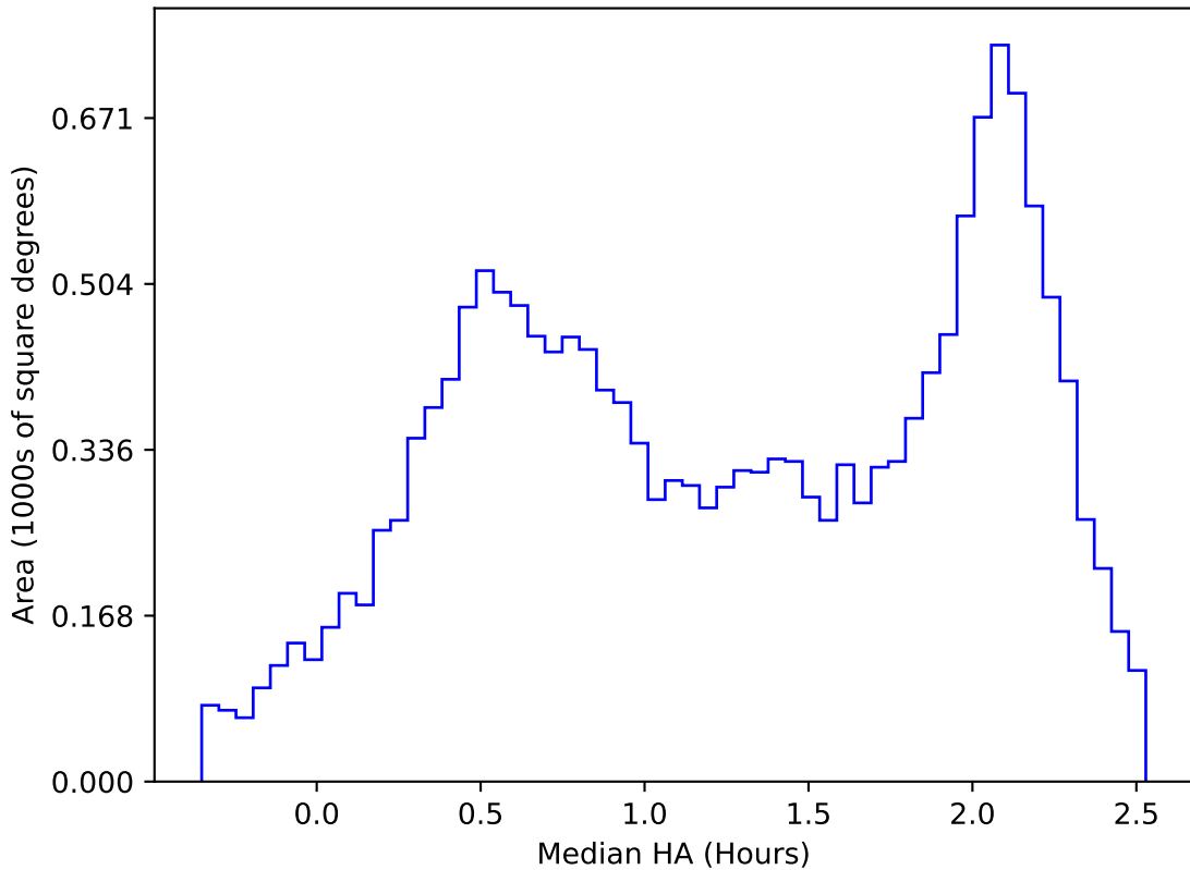
too_elab_r16_d3_giz_v3.4_10yrs WFD y band: Median HA
