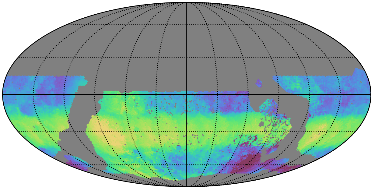
too_elab_r16_d3_giz_v3.4_10yrs WFD u band: Median HA
