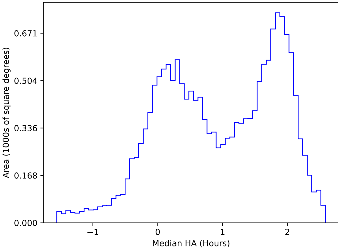
too_elab_r16_d3_giz_v3.4_10yrs WFD u band: Median HA
