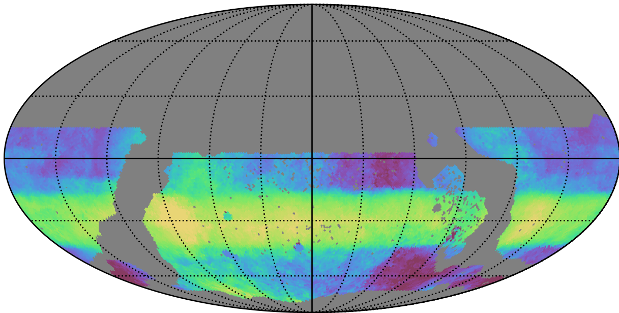
too_elab_r16_d3_giz_v3.4_10yrs WFD r band: Median HA
