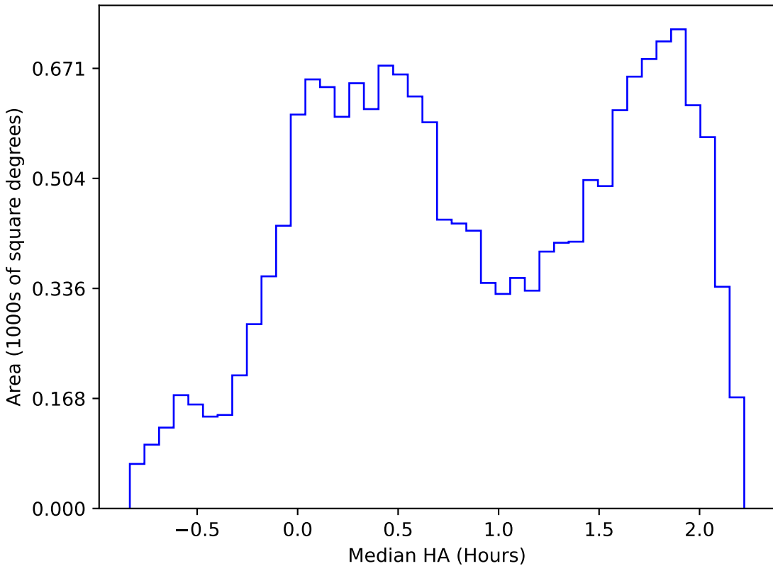
too_elab_r16_d3_giz_v3.4_10yrs WFD r band: Median HA
