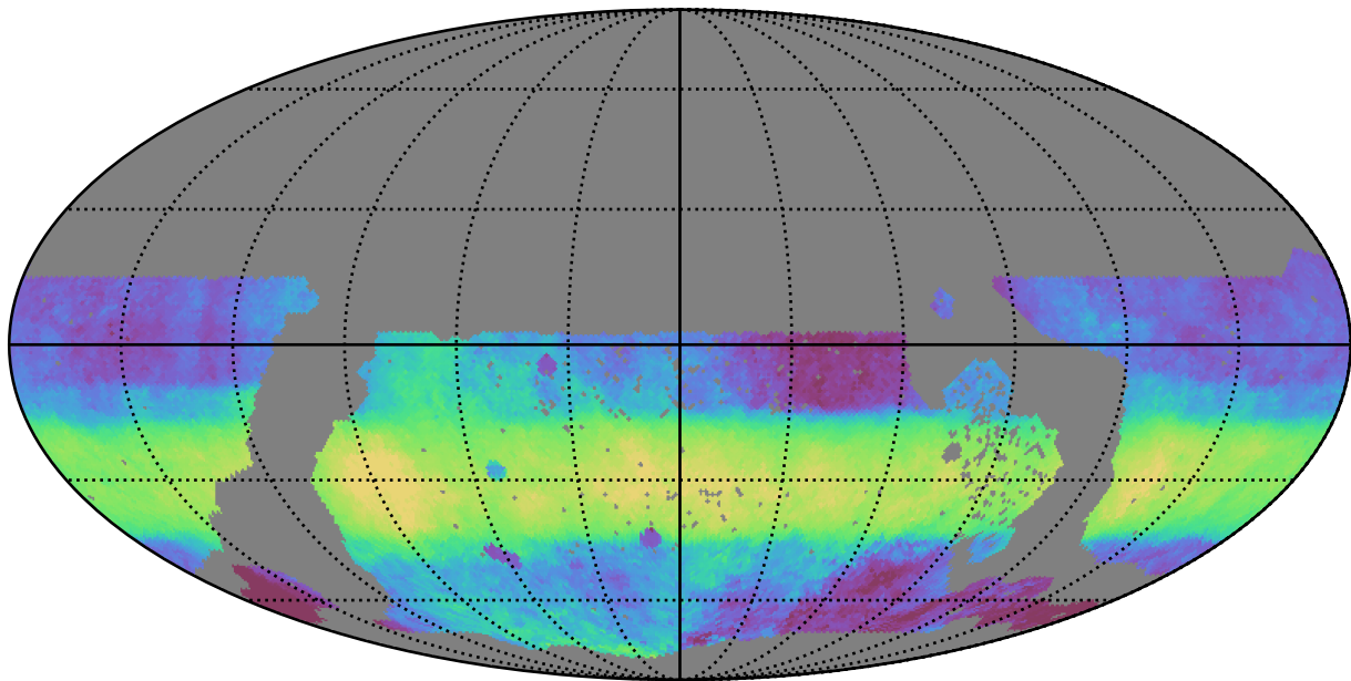
too_elab_r16_d3_giz_v3.4_10yrs WFD i band: Median HA
