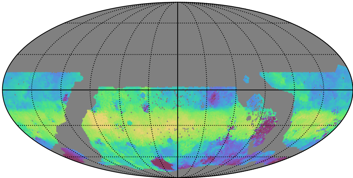
too_elab_r16_d3_giz_v3.4_10yrs WFD g band: Median HA
