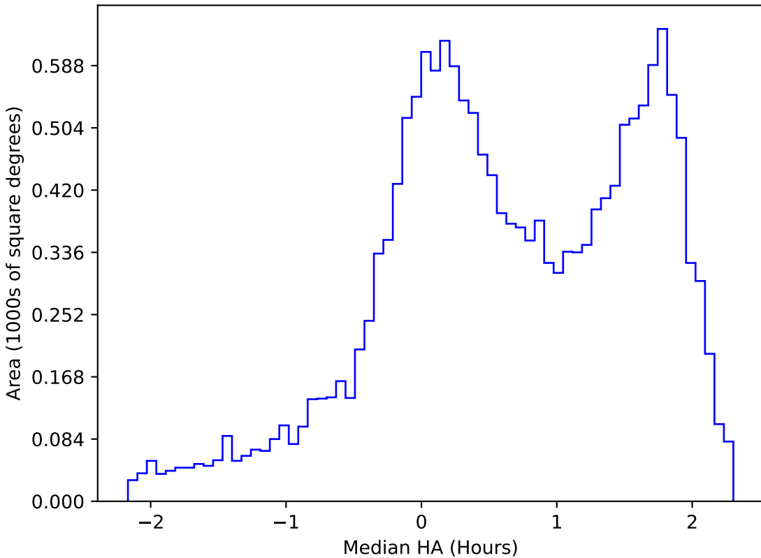
too_elab_r16_d3_giz_v3.4_10yrs WFD g band: Median HA
