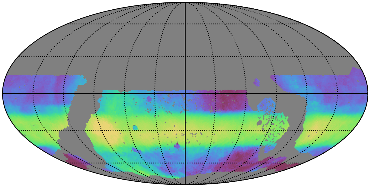
too_elab_r16_d3_giz_v3.4_10yrs WFD all bands: Median HA
