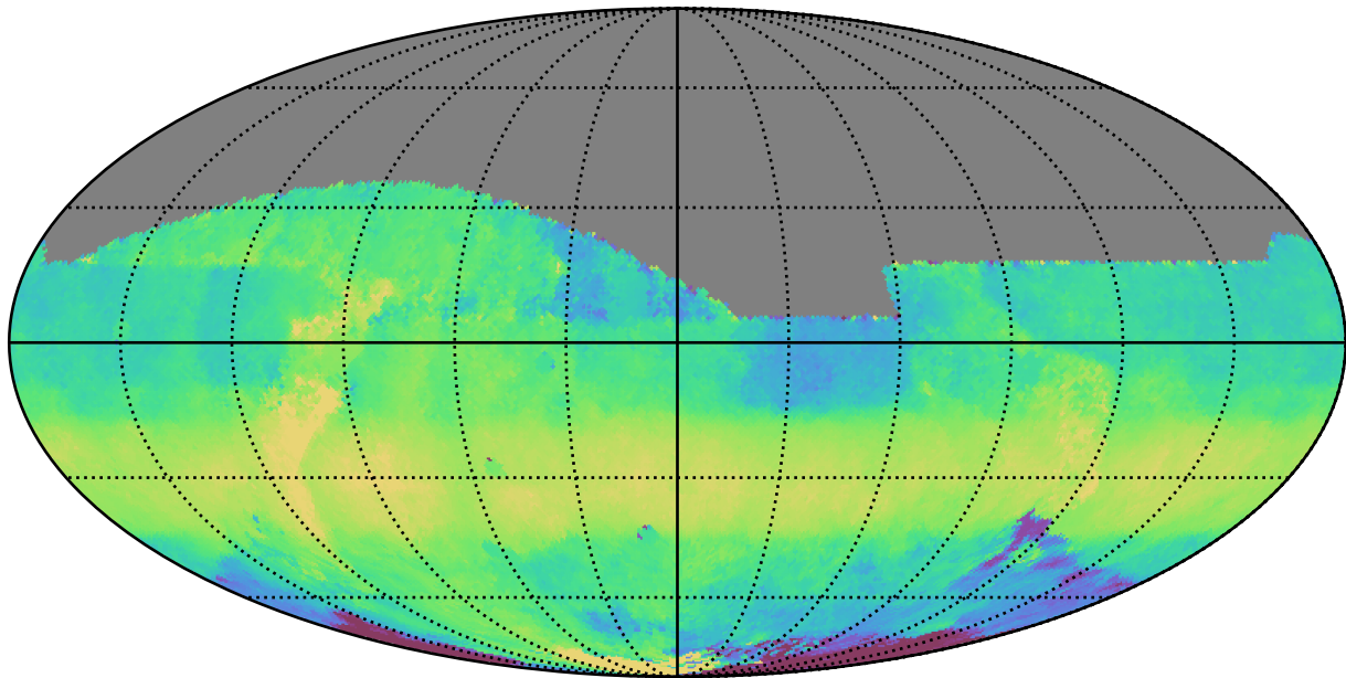
too_elab_r16_d3_giz_v3.4_10yrs All sky z band: Median HA
