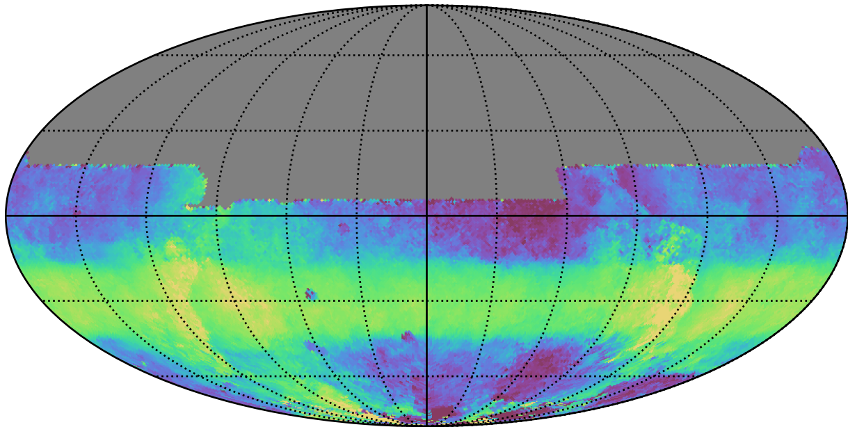
too_elab_r16_d3_giz_v3.4_10yrs All sky y band: Median HA
