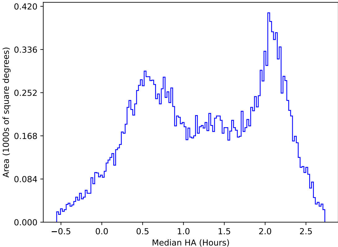
too_elab_r16_d3_giz_v3.4_10yrs All sky y band: Median HA
