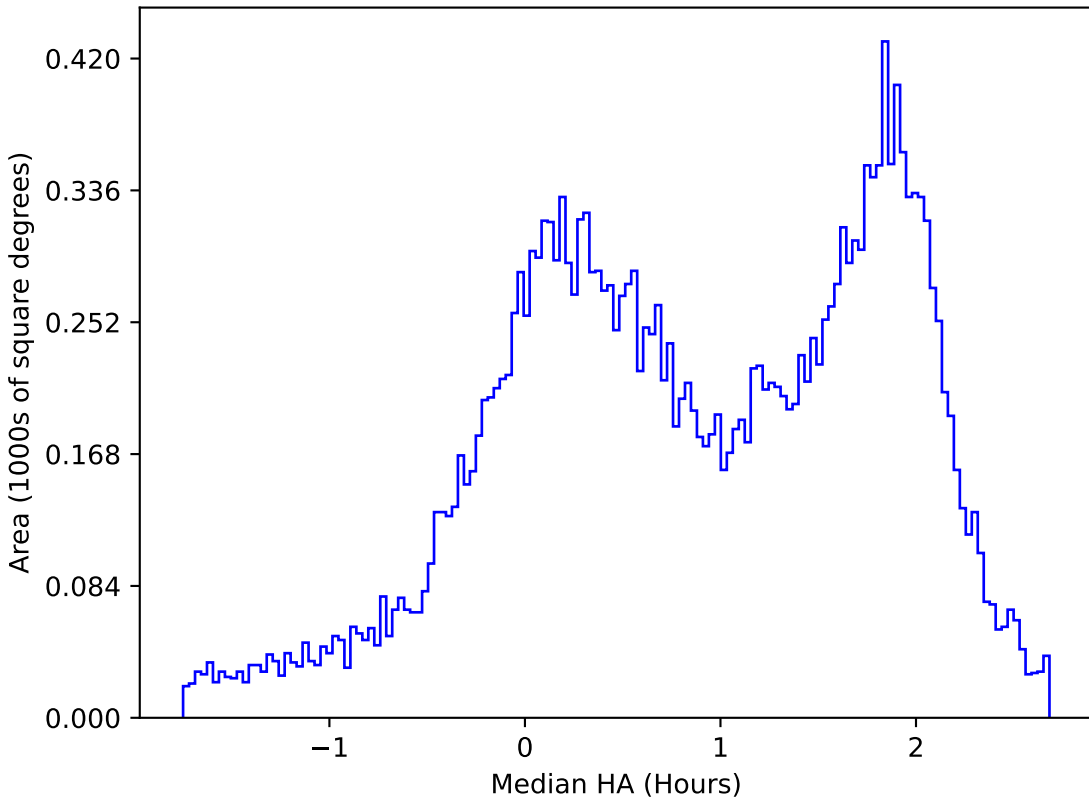
too_elab_r16_d3_giz_v3.4_10yrs All sky u band: Median HA
