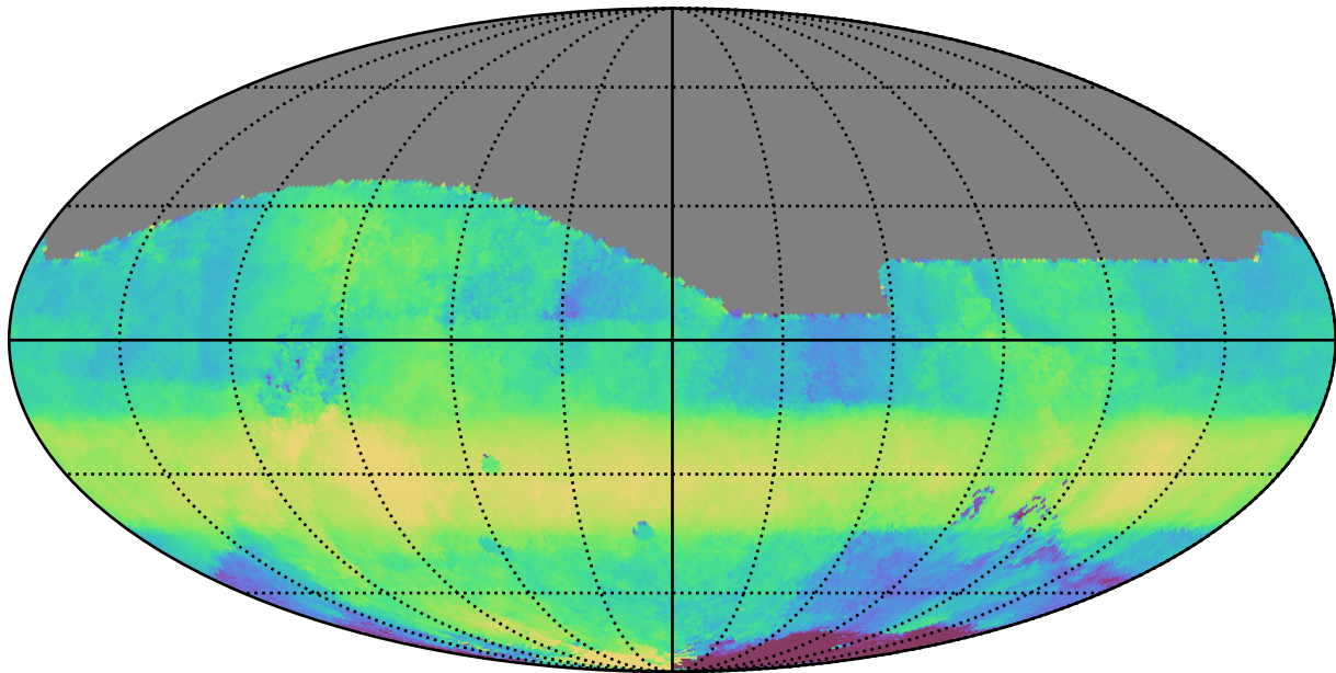
too_elab_r16_d3_giz_v3.4_10yrs All sky r band: Median HA
