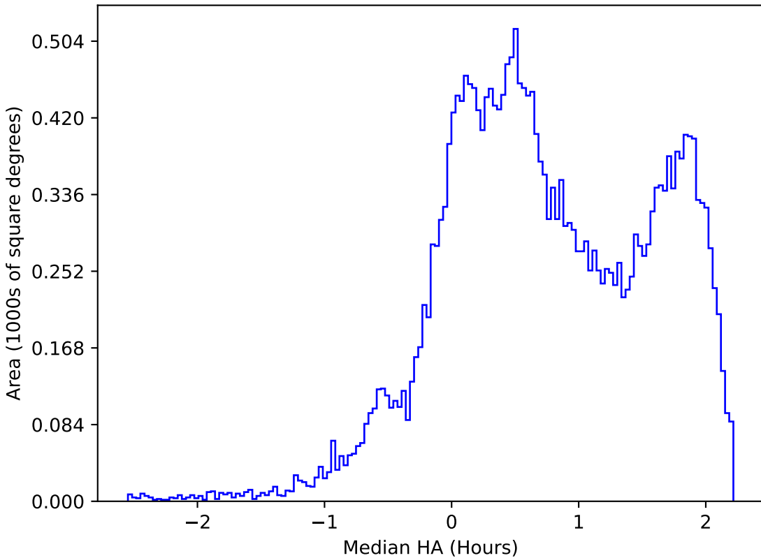
too_elab_r16_d3_giz_v3.4_10yrs All sky r band: Median HA
