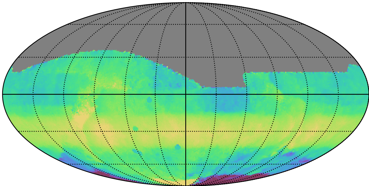
too_elab_r16_d3_giz_v3.4_10yrs All sky i band: Median HA
