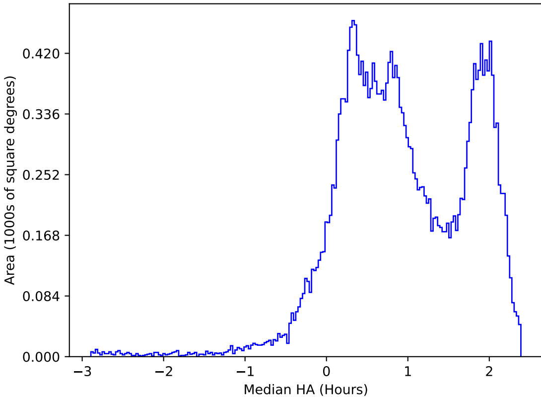
too_elab_r16_d3_giz_v3.4_10yrs All sky i band: Median HA
