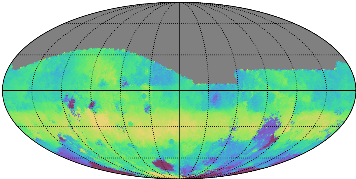
too_elab_r16_d3_giz_v3.4_10yrs All sky g band: Median HA
