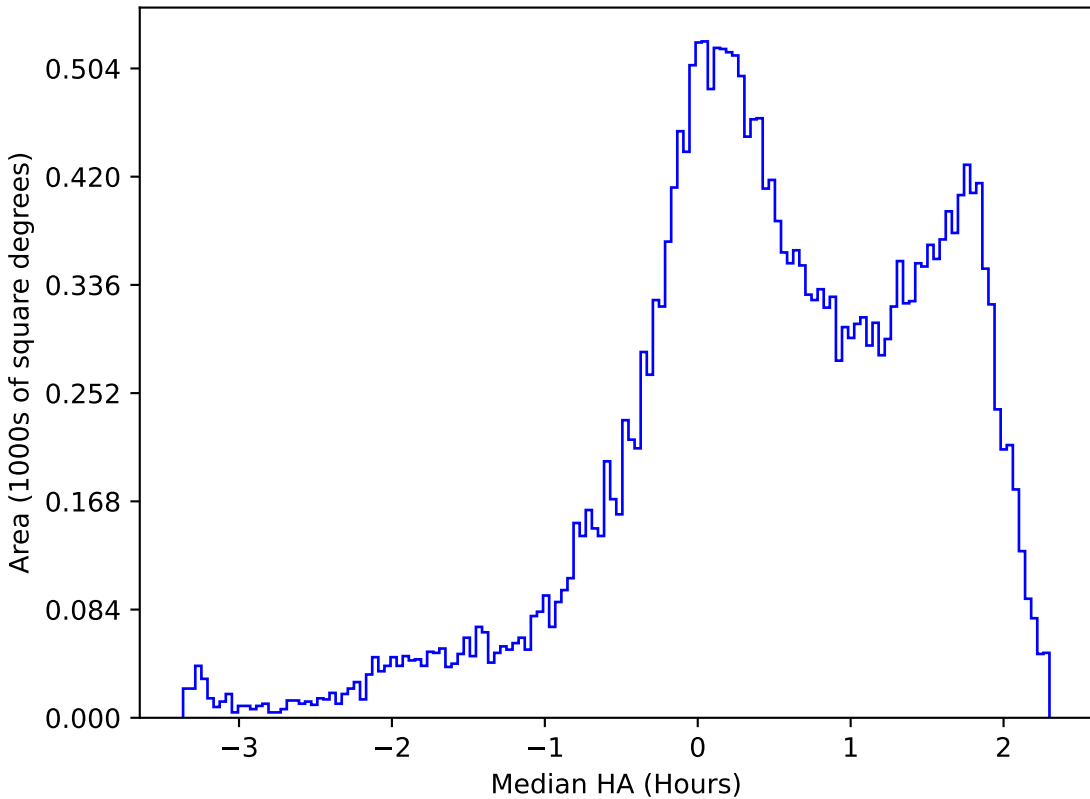
too_elab_r16_d3_giz_v3.4_10yrs All sky g band: Median HA
