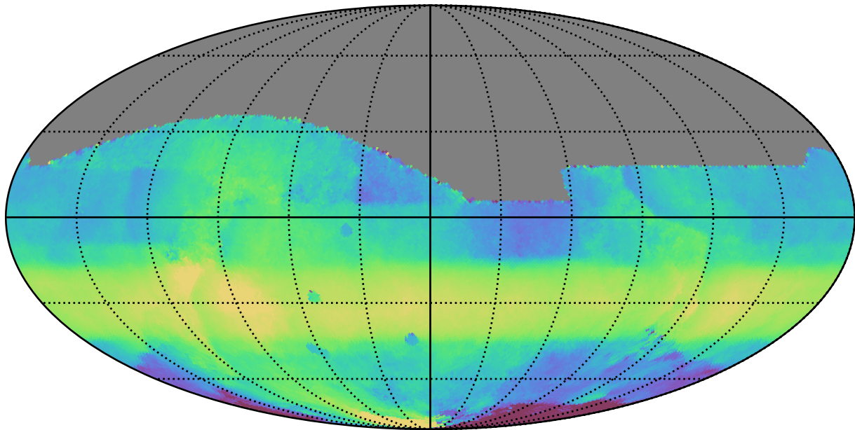
too_elab_r16_d3_giz_v3.4_10yrs All sky all bands: Median HA
