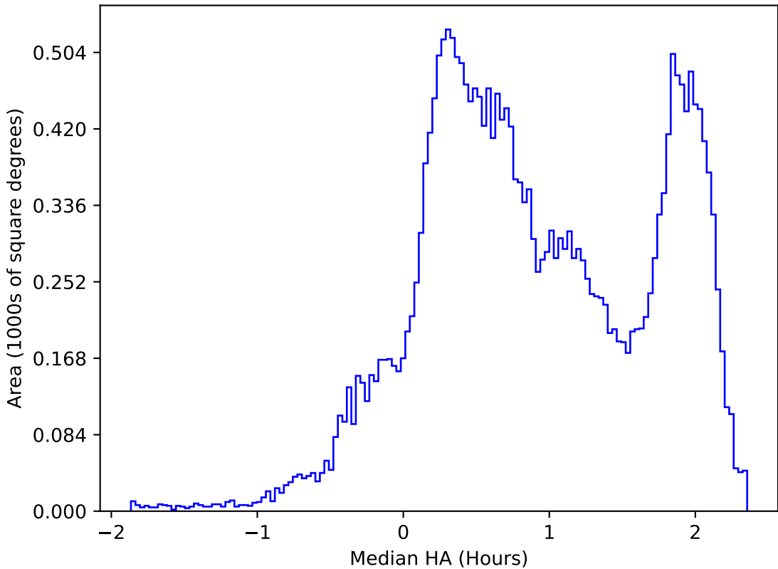
too_elab_r16_d3_giz_v3.4_10yrs All sky all bands: Median HA
